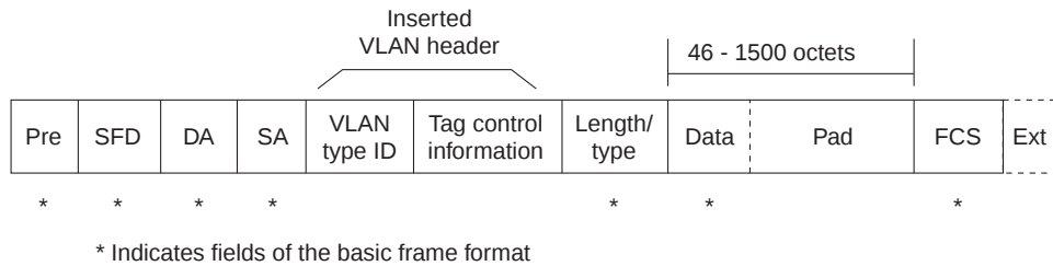
Figure 7-11 VLAN-Tagged Frames Are Identified When the MAC Finds the LAN Type Value in the Normal Length/Type Field Location
