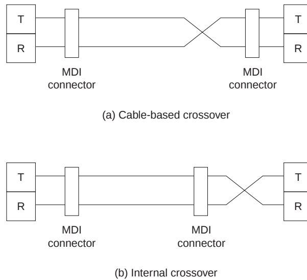
Figure 7-26 Alternative Ways for Implementing the Link Crossover Requirement
